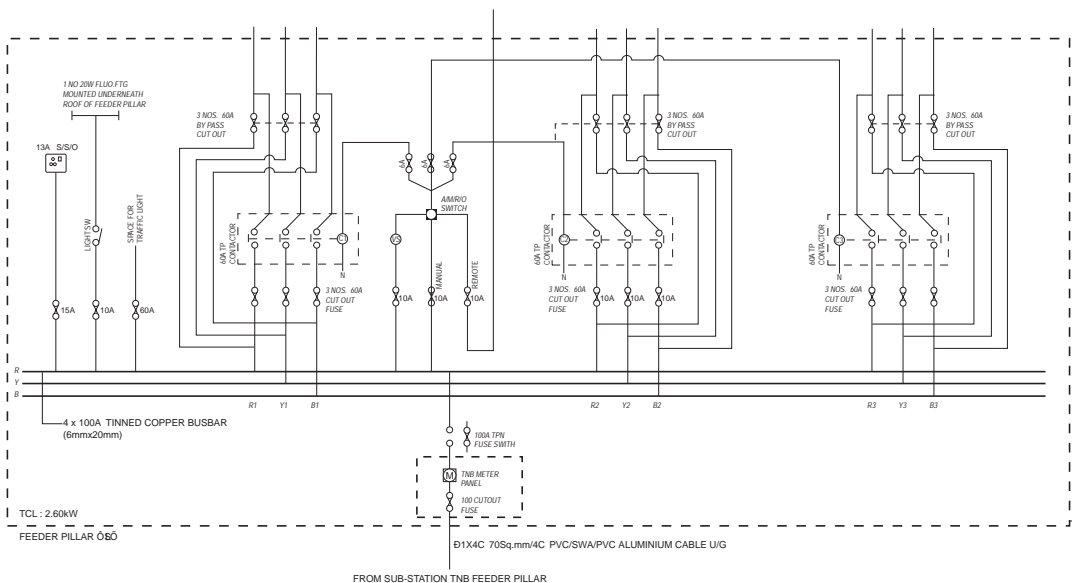
Schematic drawing
